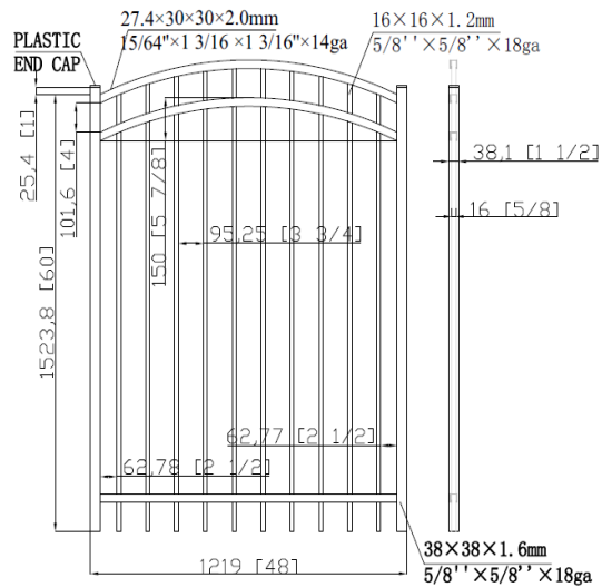
N02873 HGX 4'Wx5'H 3R Univ ASWG Blk 5/8" x 18ga PB Arch (residential arch gate 3-rail flat top/extended bottom)
